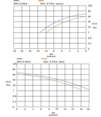
GB series vortex air pump performance curve (for reference only, do not take it for testing standard)
